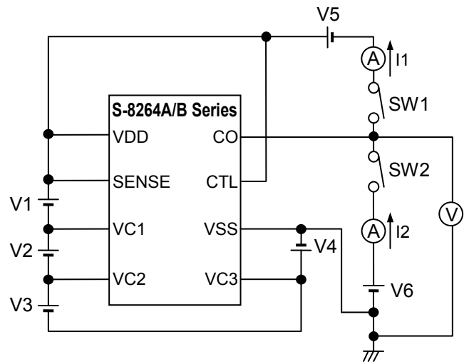
Test Circuit 6
