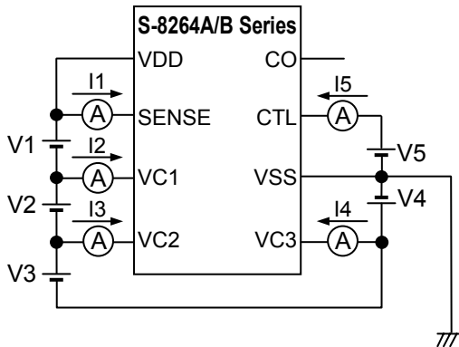
Test Circuit 5
