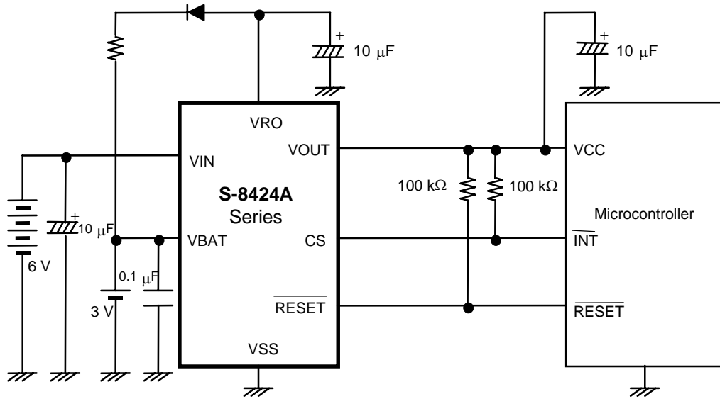
Figure 24 Application Circuit 2
