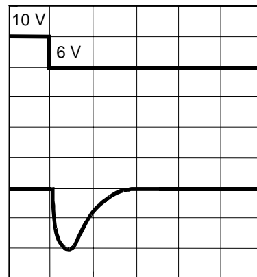
Figure 16 Ringing Waveform of Power Supply Variation (VOUT Pin)
