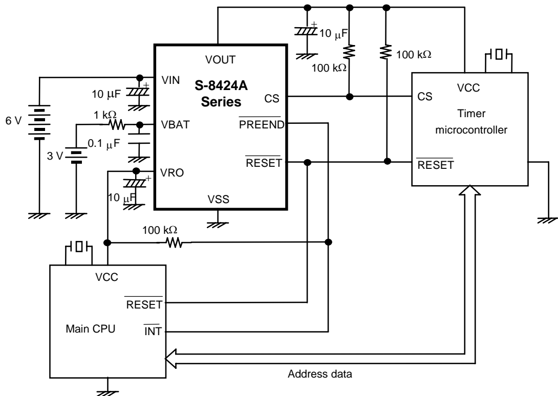
Figure 23 Application Circuit 1
