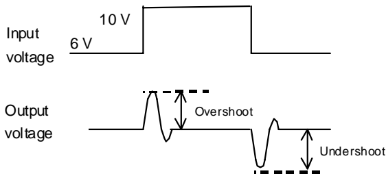
Figure 14 Power Supply Variation: 6 V and 10 V Square Waves
