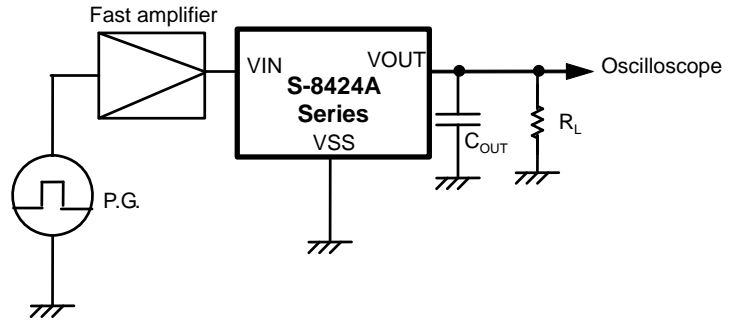
Figure 11 Test Circuit
