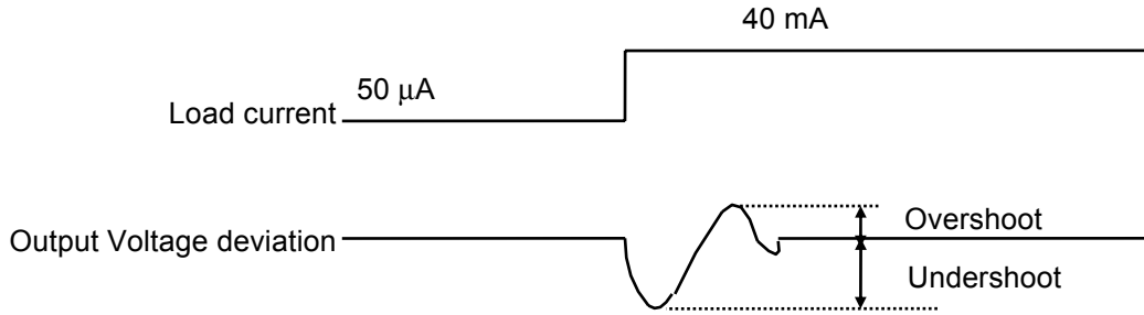
Figure 30 Output voltage fluctuation due to a change in the load current
