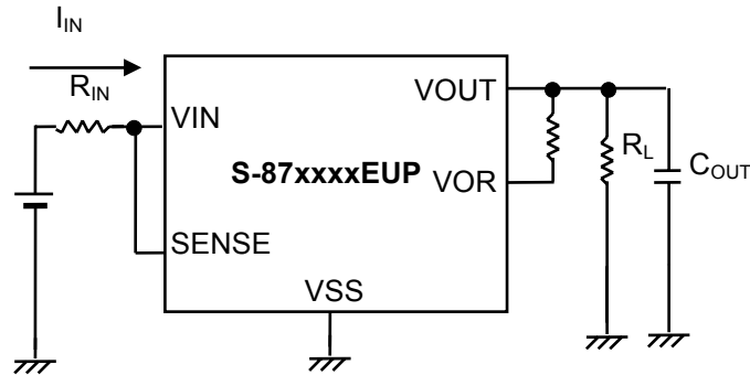
Figure 23 Attention connecting example 2
