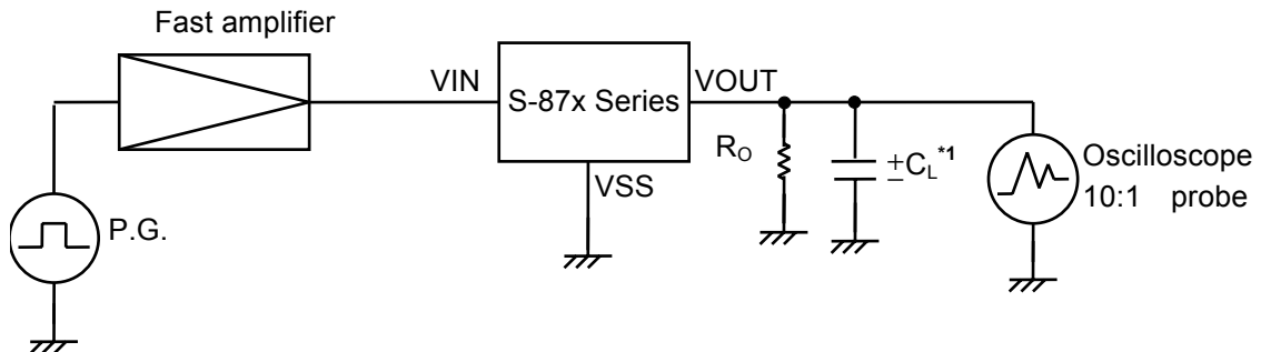
Figure 26 Rectangular wave from 0 V to 10 V (Type 2)
