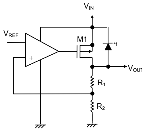
Figure 17 Voltage regulator circuit
