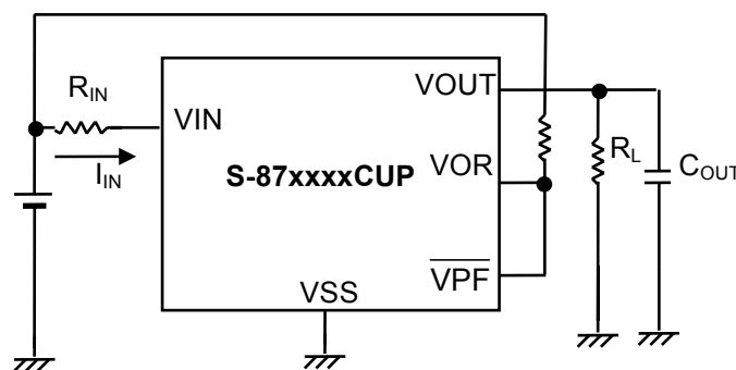
Figure 22 Attention connecting example 1
