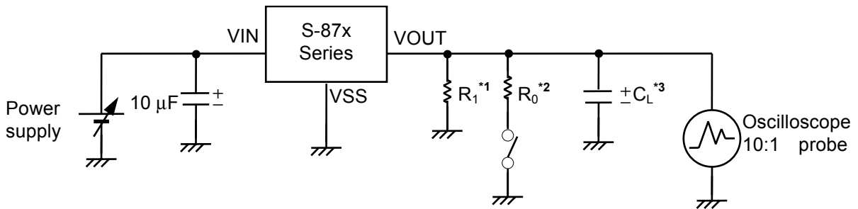
Figure 30 Output voltage fluctuation due to a change in the load current
