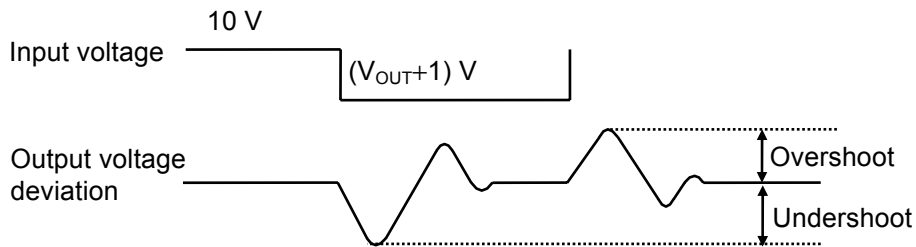
Figure 25 Rectangular wave between ( V_{OUT}+1 ) V and 10 V (Type 1)
