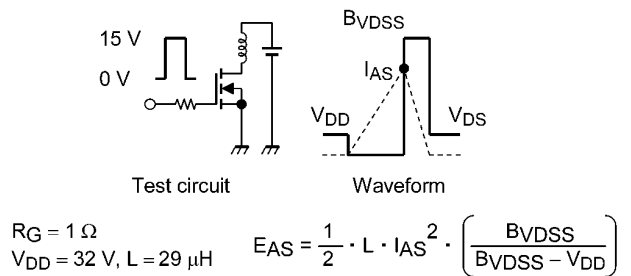
Fig. 9.16 Test Circuit/Waveform
