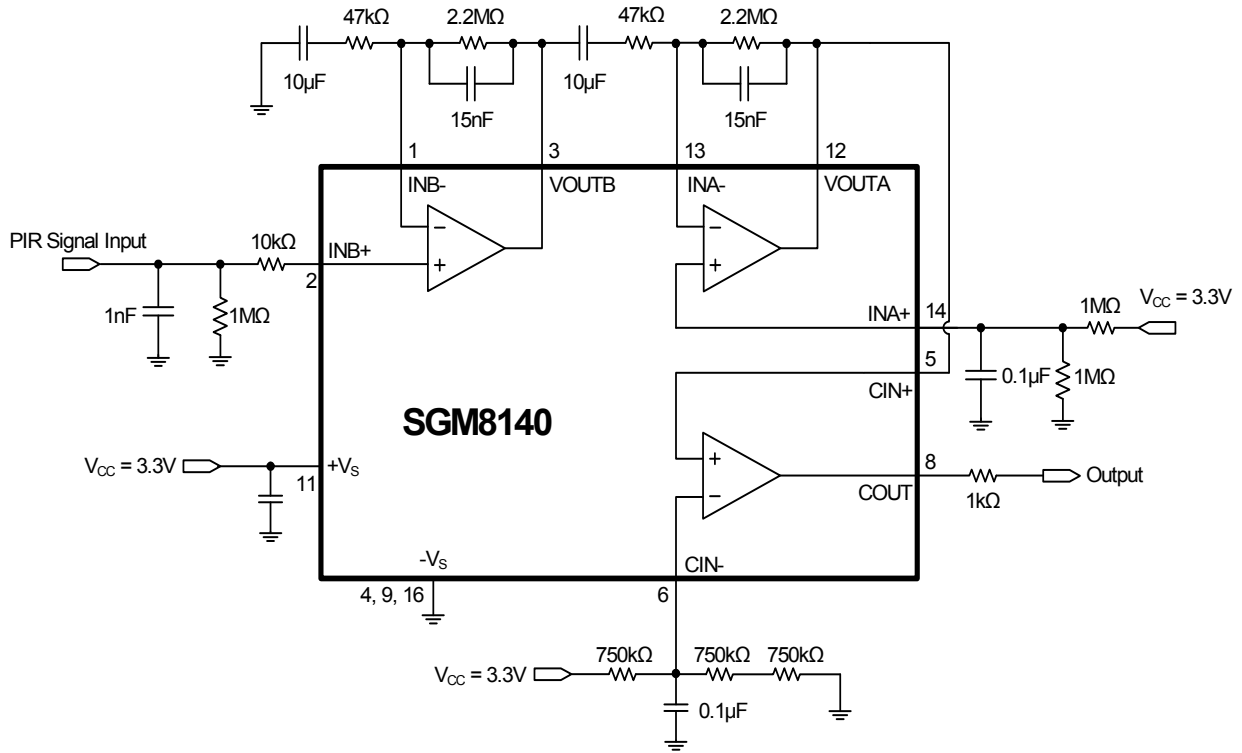
Figure 1. Application Circuit for PIR Sensor
